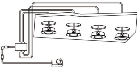
Recessed Mounting
