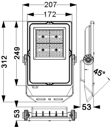
Mounting Holes
