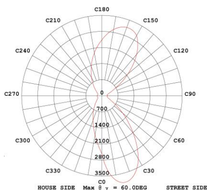
MAX INTENSITY CONE SURFACE DISTRIBUTION DIAGRAM
