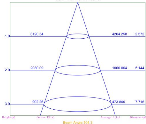
Illuminance-Distance Curve
