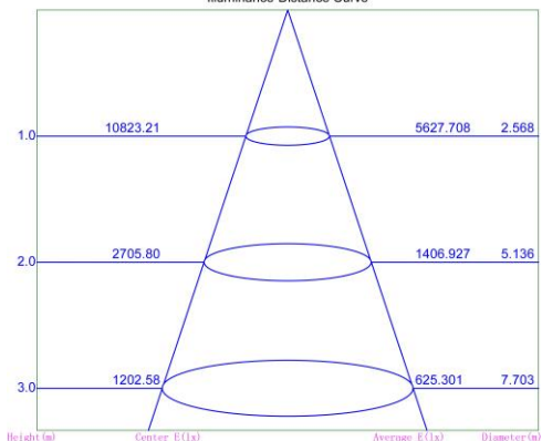
Illuminance-Distance Curve
