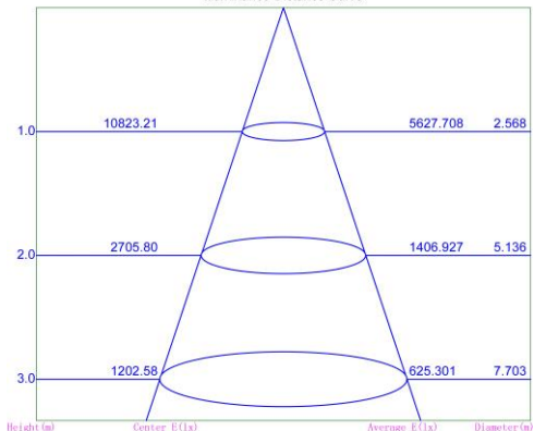
Illuminance-Distance Curve
