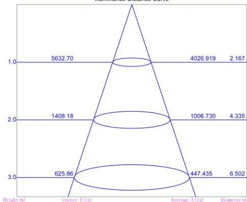
Illuminance-Distance Curve
