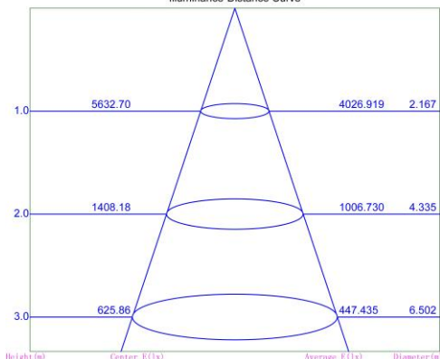
Illuminance-Distance Curve
