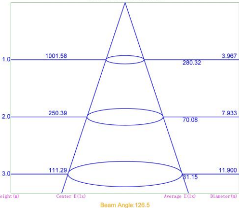
Illuminance-Distance Curve
